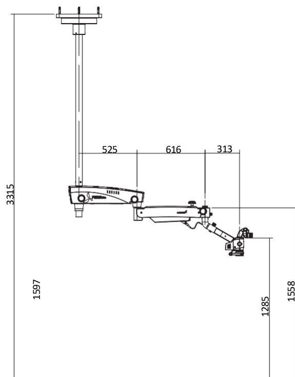
CEILING MOUNT
